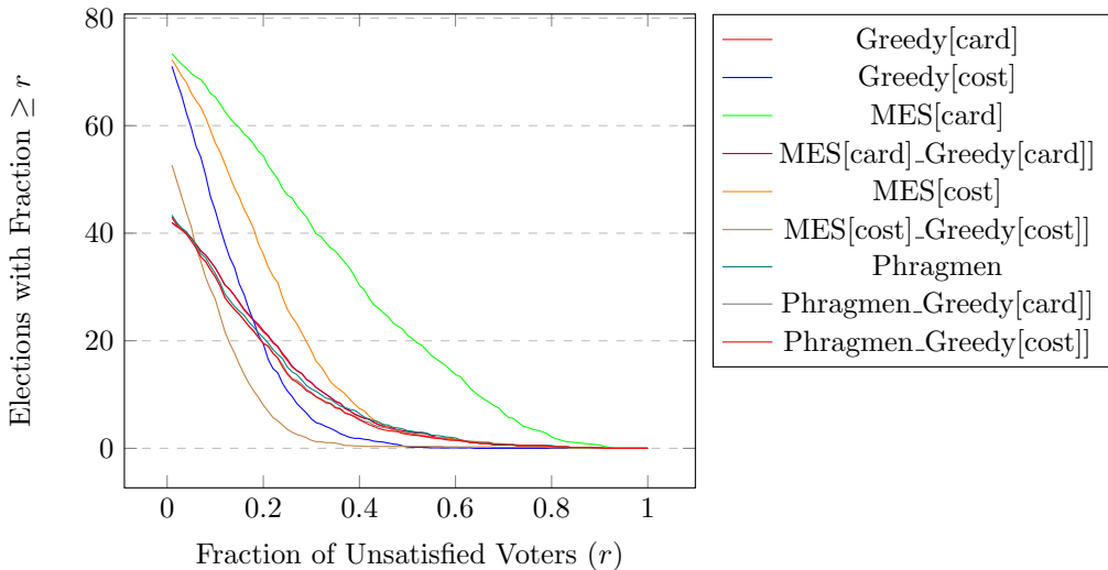
EJR[cost] Unsatisfied Voter Fraction Distribution
