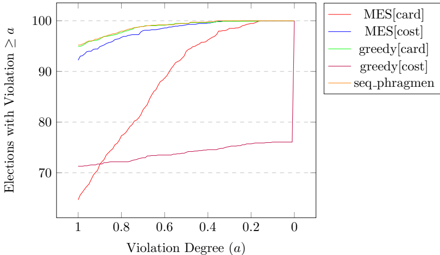
EJR[cost] Violation Degree Distribution
