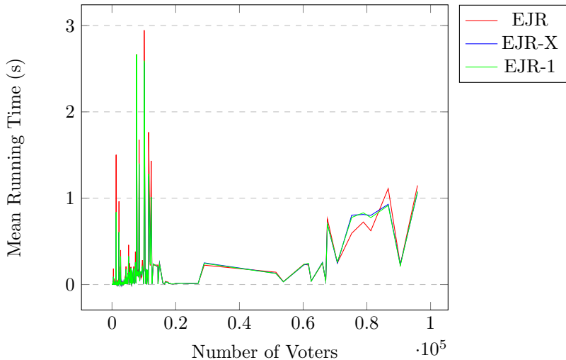
EJR Running Time vs Number of Voters (bucket size=50)
