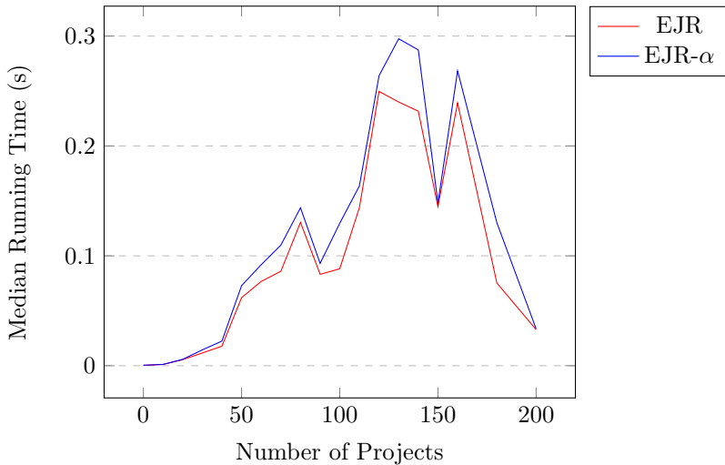
EJR Running Time vs Number of Projects (EJR vs EJ R -exit-early) (bucket size=10)
