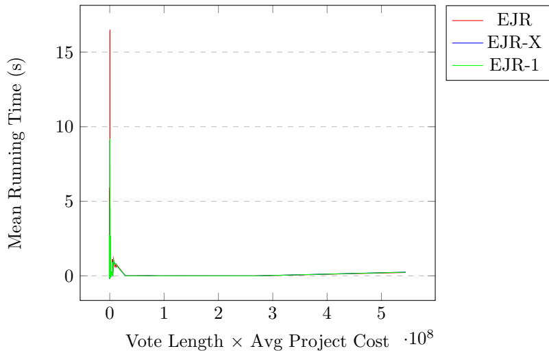
EJR Running Time vs Vote Length \times Avg Project Cost (bucket size=5)
