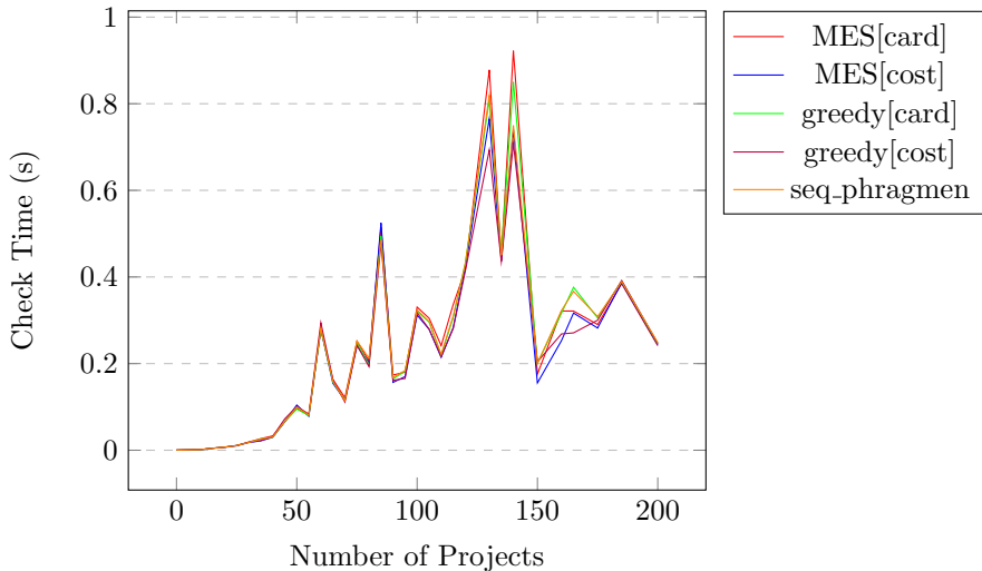
EJR[ cost ] Check Time vs Number of Projects
