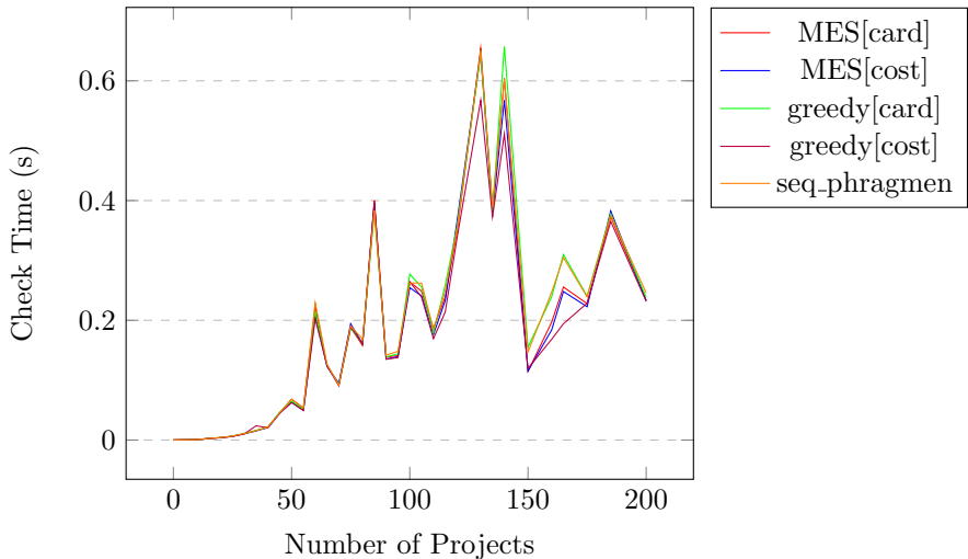
EJR[card] Check Time vs Number of Projects
