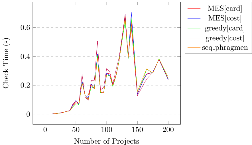
EJR-X[ cost ] Check Time vs Number of Projects
