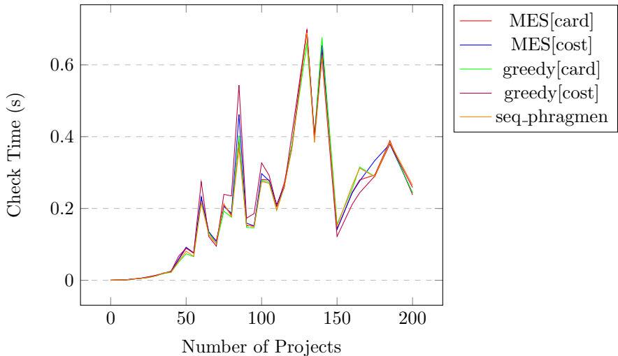
EJR-1[ cost ] Check Time vs Number of Projects
