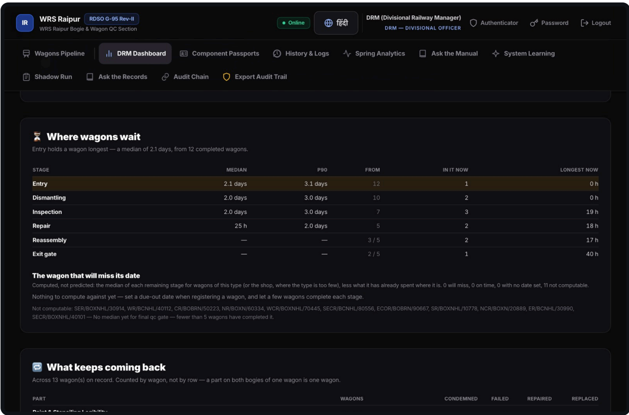
dashboard lower
