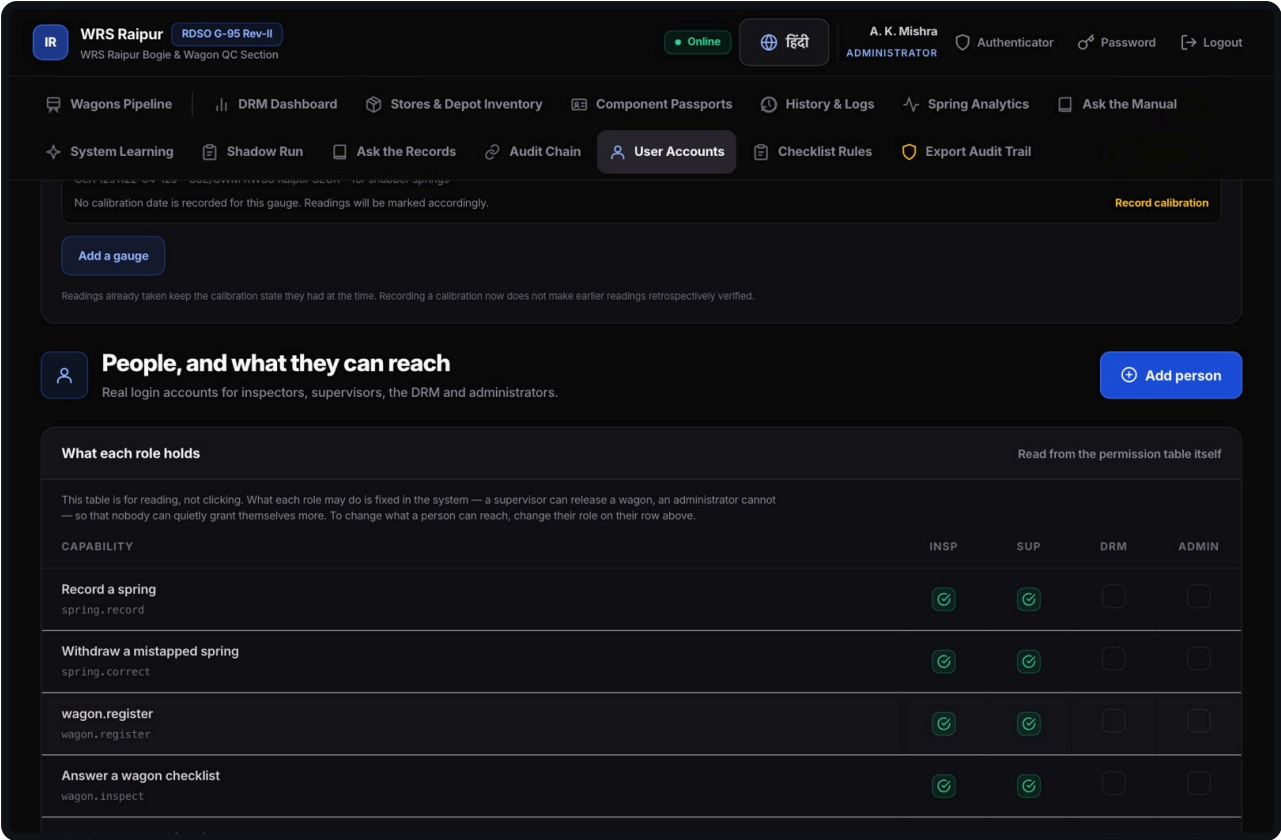
role matrix
