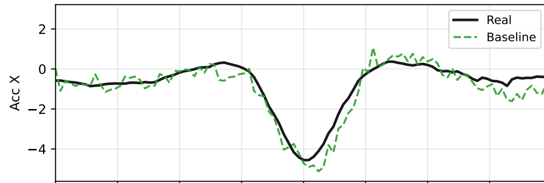
With MSE Loss (MSE = 0.260)
