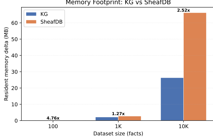
Figure 5: Resident memory delta from inserting N facts. SFDB uses 1.3–4.8 \times more memory than the KG baseline at every scale measured.
