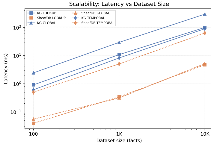
Figure 6: Scalability: latency versus dataset size (log-log).
