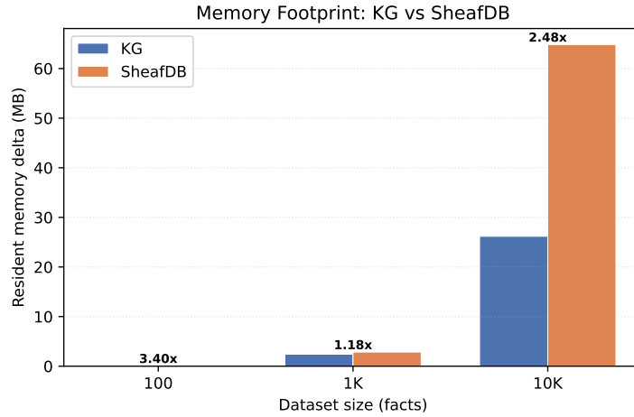
Figure 5: Resident memory delta from inserting N facts. SFDB uses 1.2–3.4 \times more memory than the KG baseline at every scale measured.
