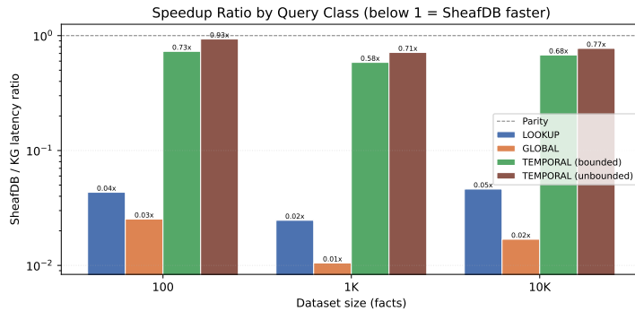
Figure 4: Ratio of SFDB to KG latency across query classes. All values are below one: SFDB is faster on every class at every scale measured.
