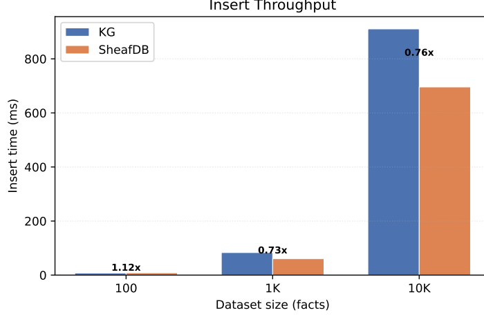
Figure 2: Insert throughput. SFDB is close to parity with the KG baseline across all three scales, with the ratio annotated above each bar.
