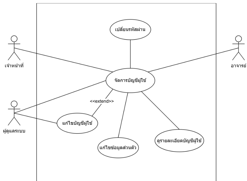
Use Case Diagram: User Account (UC-02.1)
