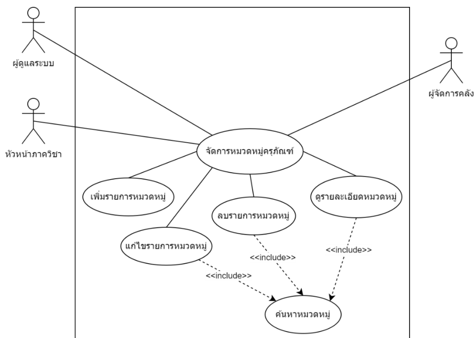
Use Case Diagram: Manage Category (UC-07)
