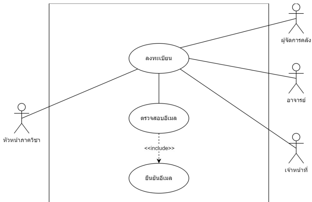
Use Case Diagram: Register (UC-01.1)
