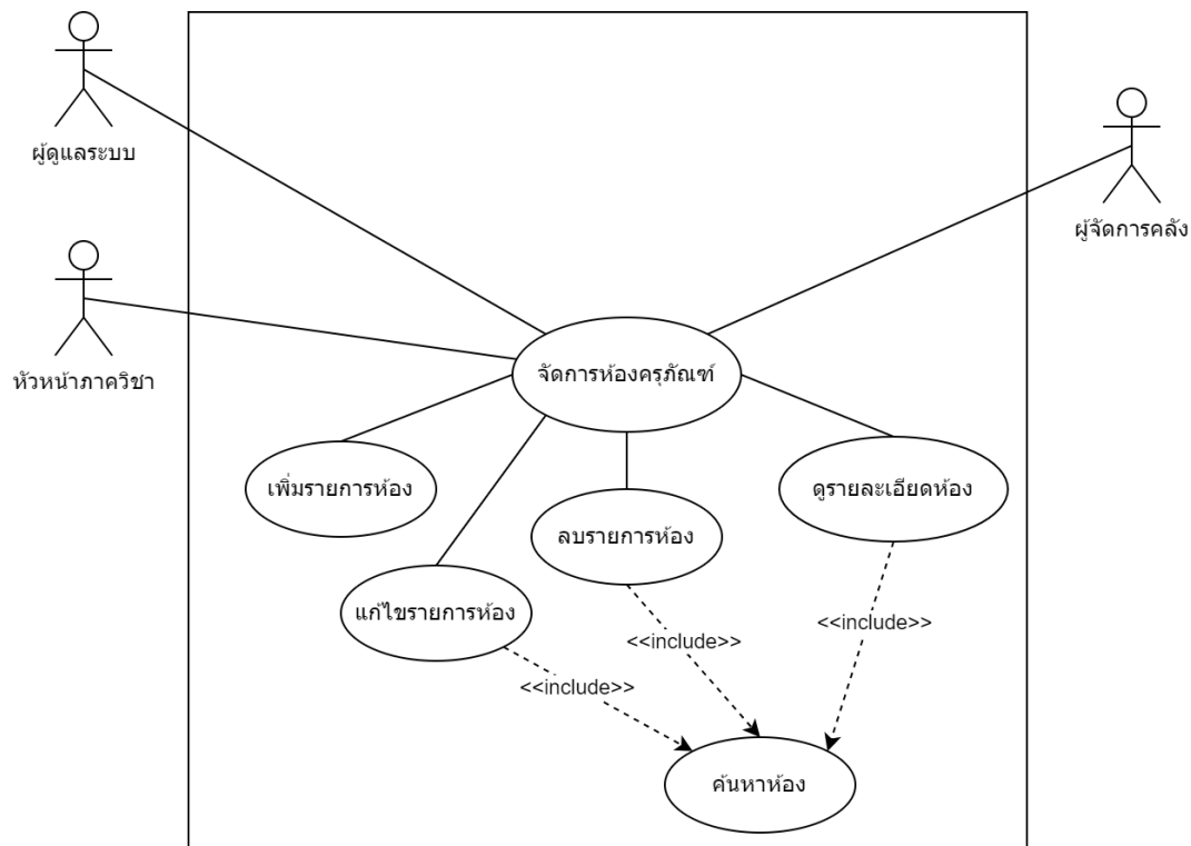
Use Case Diagram: Manage Rooms (UC-06)
