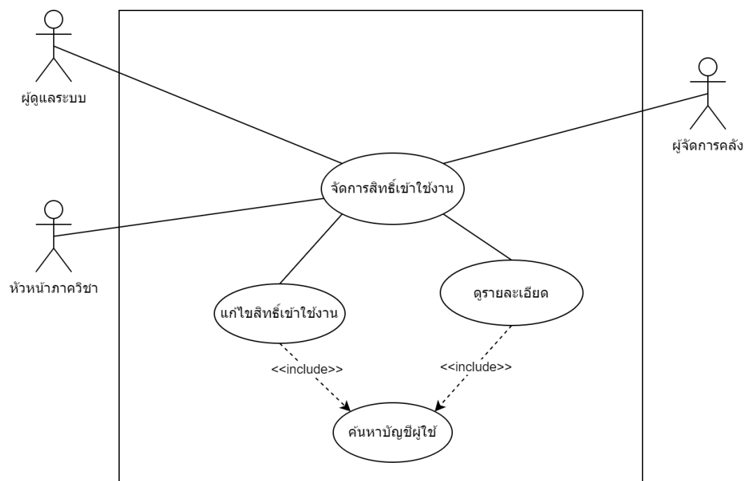
Use Case Diagram: Manage Permission (UC-03)
