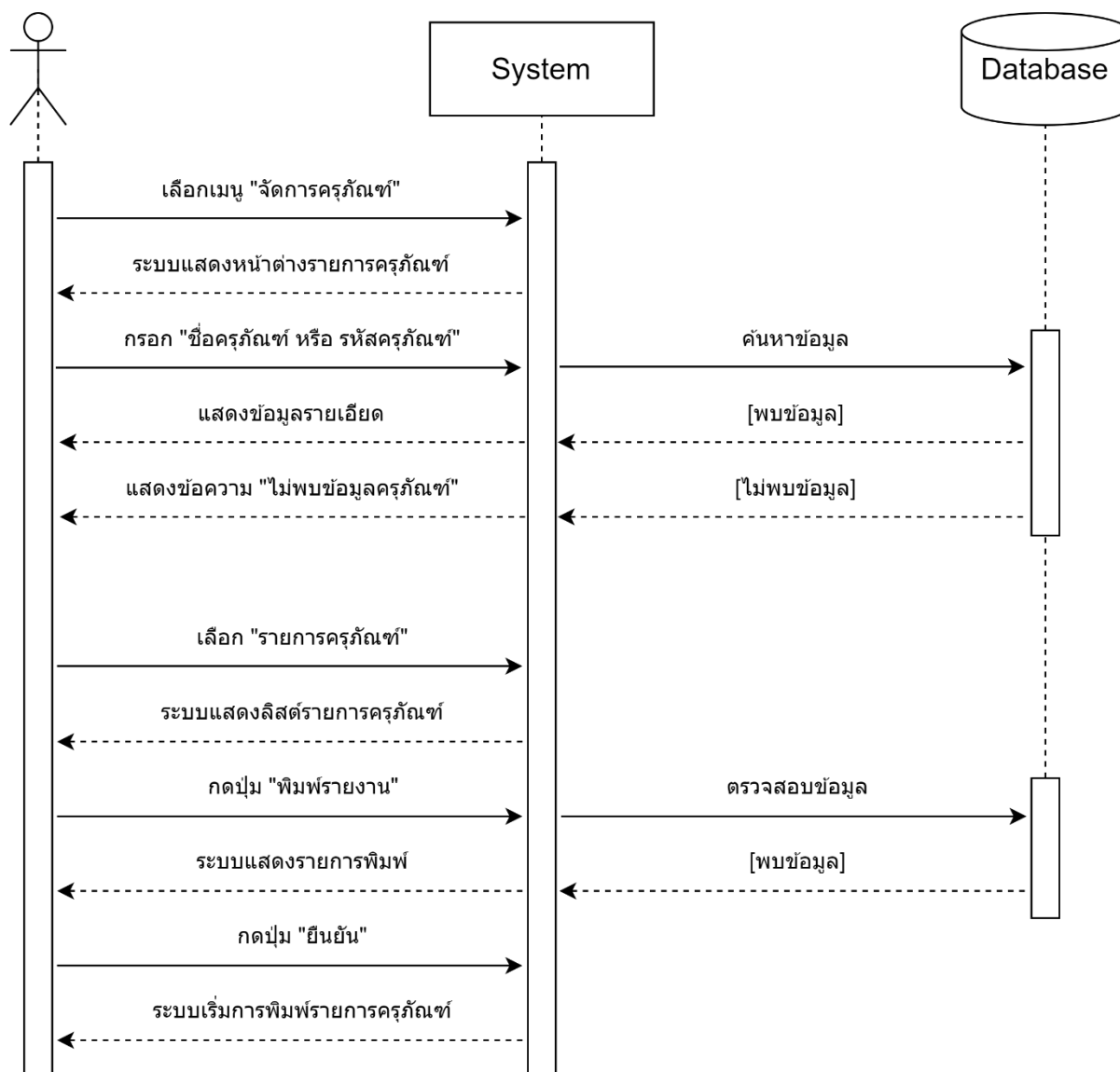
Sequence Diagram: Equipment Data (UC-05)
