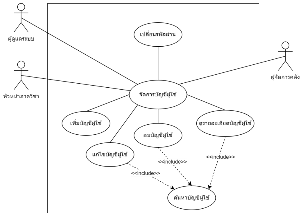
Use Case Diagram: Manage Account (UC-02)
