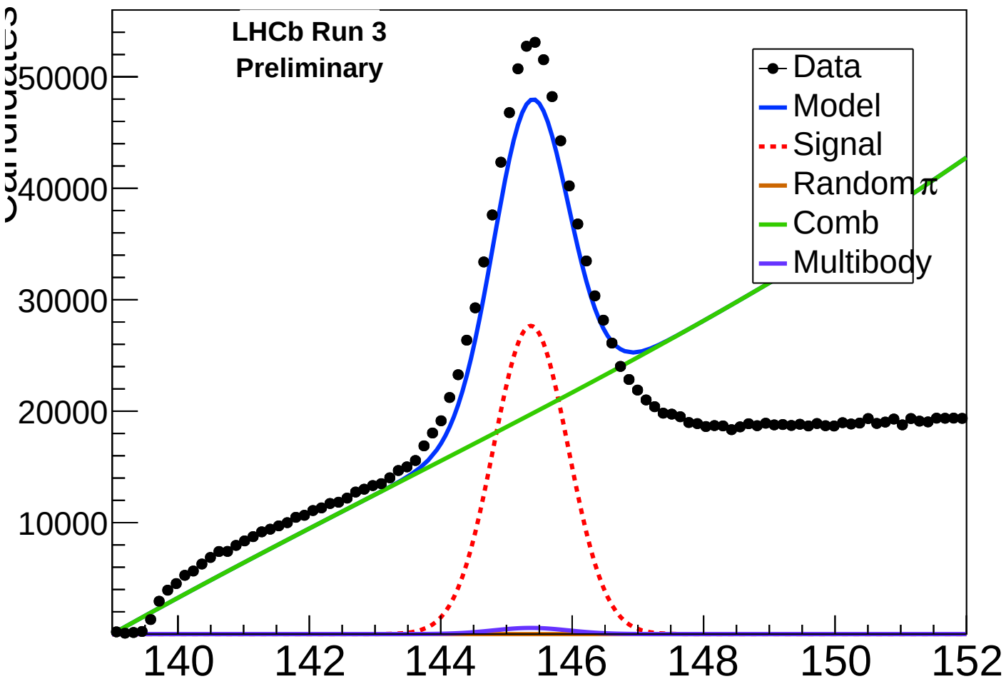
A RooPlot of "deltaM"
