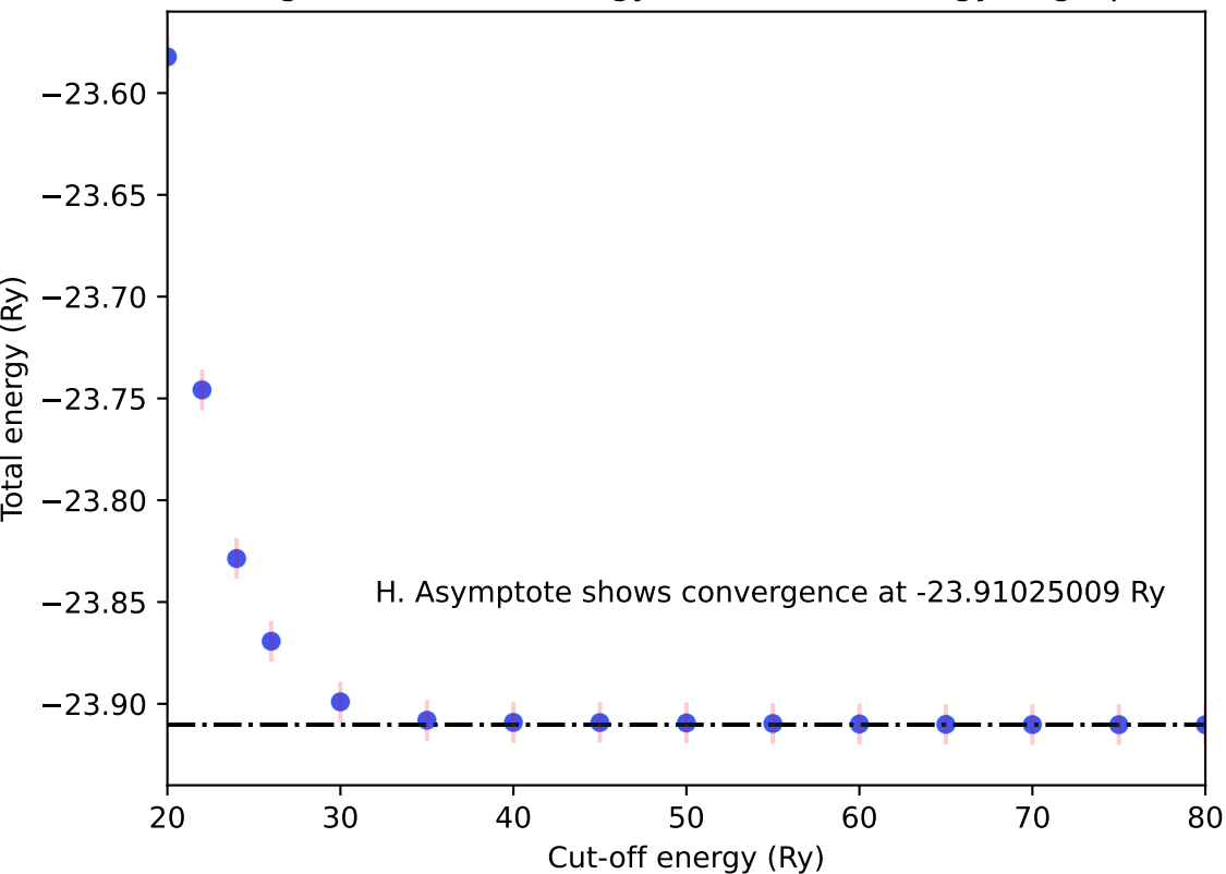
Convergence of total energy with cut-off energy of graphene
