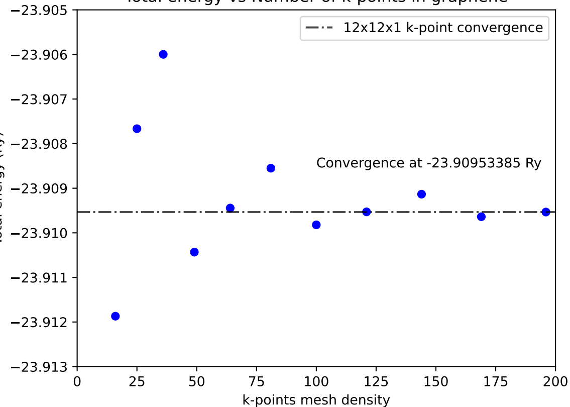
Total energy vs Number of k-points in graphene
