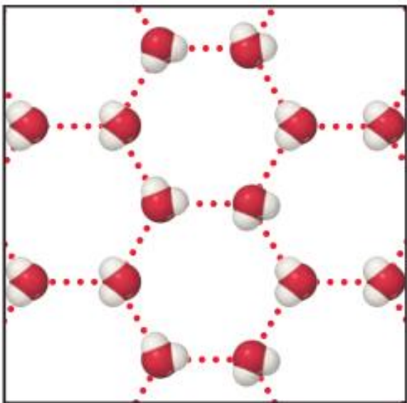
Ice
