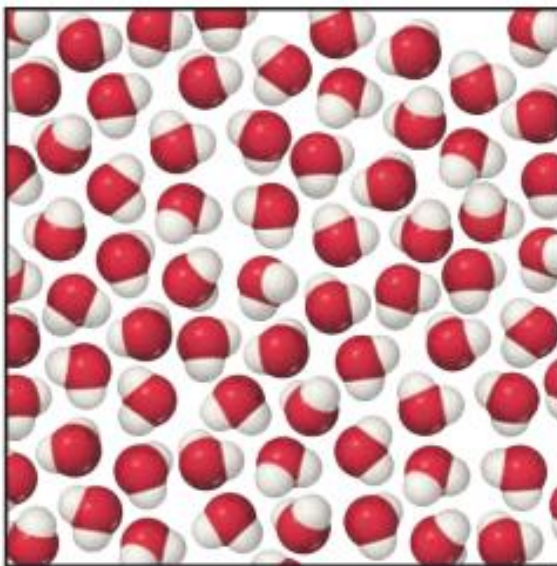
Liquid water
