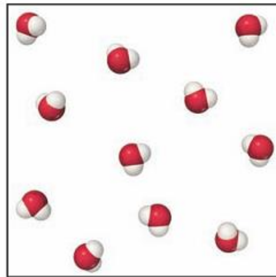
Water vapor
