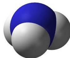
Ammonia, \text{NH}_3
