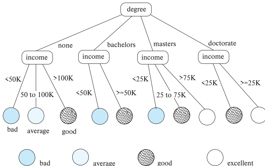
Figure 11.11 Classification tree.
