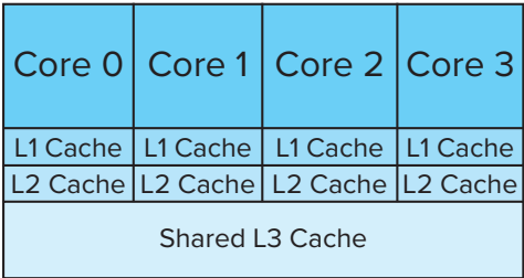
Figure 20.7 Multilevel cache system.
