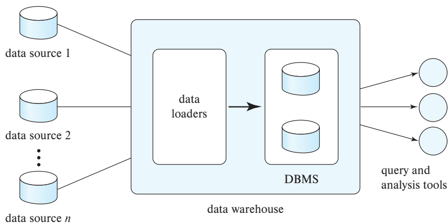
Figure 11.1 Data-warehouse architecture.
