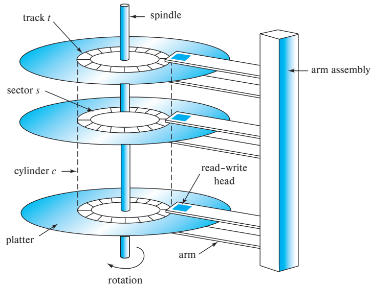
Figure 12.2 Schematic diagram of a magnetic disk.
