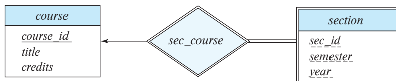
Figure 6.14 E-R diagram with a weak entity set.
