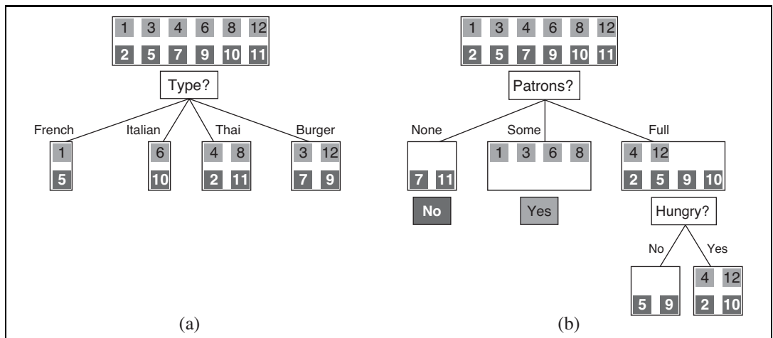
Figure 18.4 Splitting the examples by testing on attributes. At each node we show the positive (light boxes) and negative (dark boxes) examples remaining. (a) Splitting on Type brings us no nearer to distinguishing between positive and negative examples. (b) Splitting on Patrons does a good job of separating positive and negative examples. After splitting on Patrons , Hungry is a fairly good second test.
