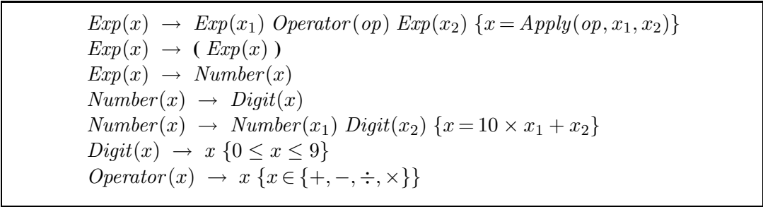
Figure 23.8 A grammar for arithmetic expressions, augmented with semantics. Each variable x_i represents the semantics of a constituent. Note the use of the \{test\} notation to define logical predicates that must be satisfied, but that are not constituents.
