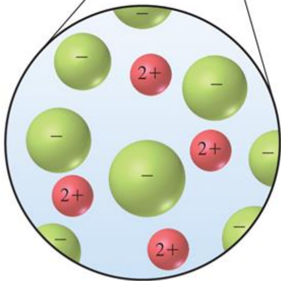
A strong electrolyte
