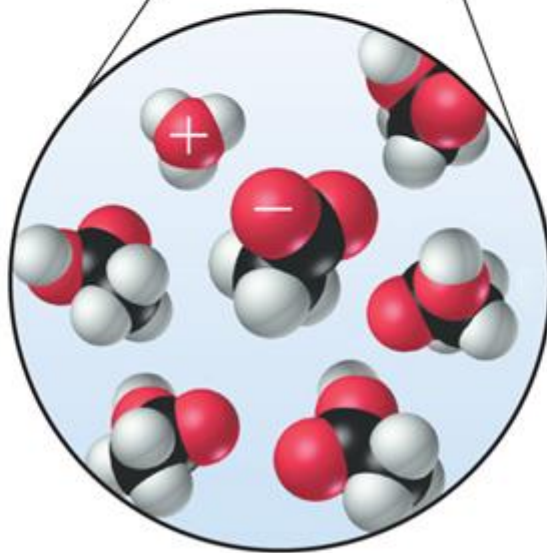
A weak electrolyte
