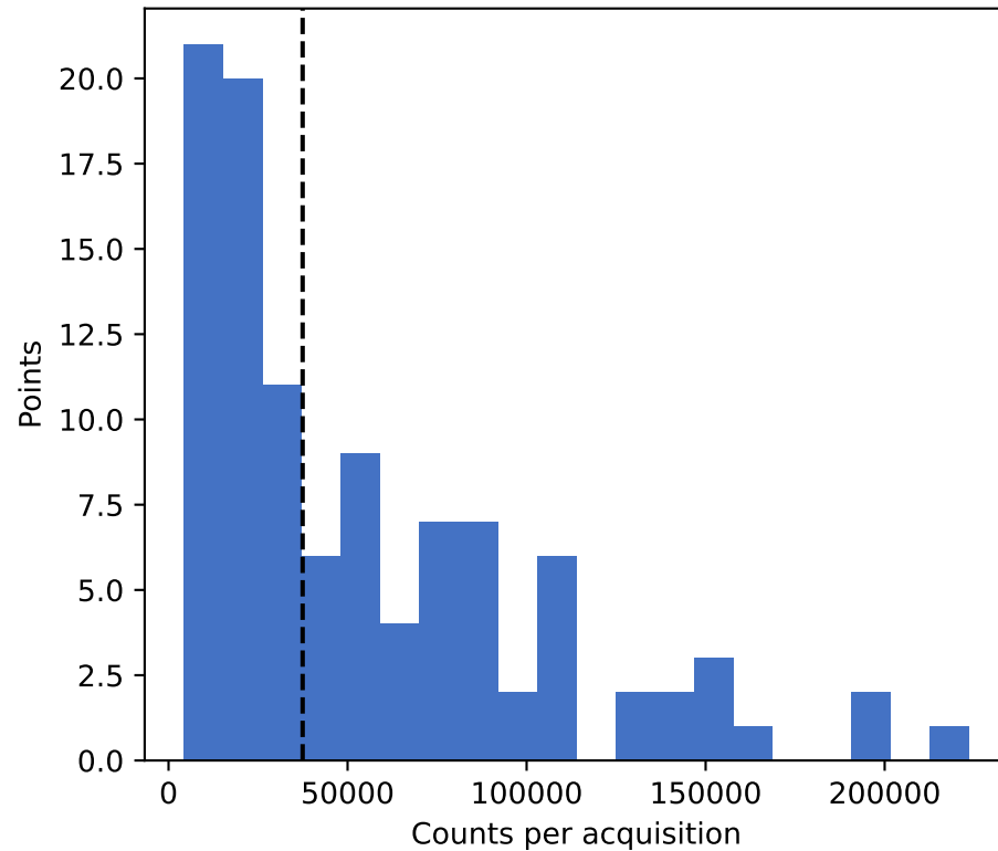
Per-point counts
