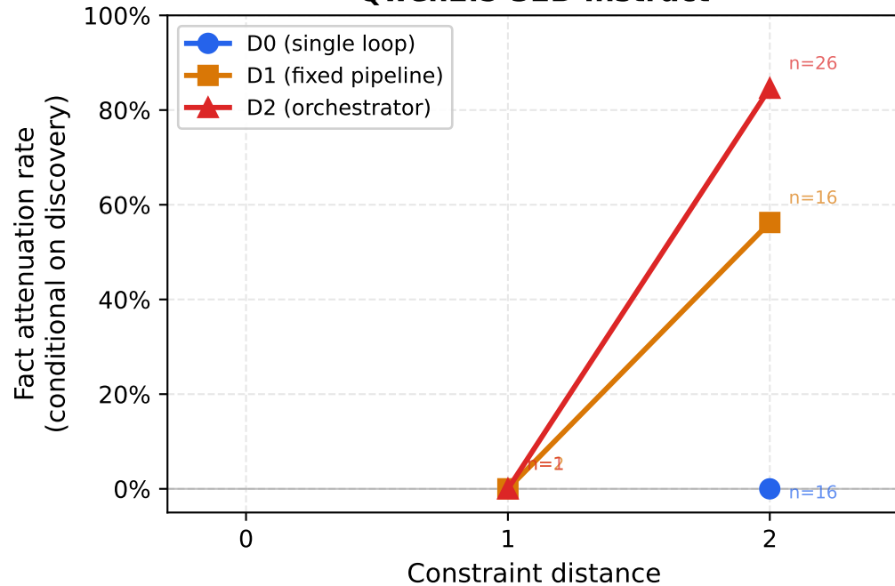
Qwen2.5-32B-Instruct
