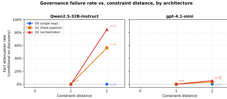
Figure 1: Fact attenuation rate (conditional on discovery) vs. constraint distance, per arm and model. D0 is structurally zero; both models show a monotone increase with decomposition depth, with gpt-4.1-mini attenuating far less at each level.
