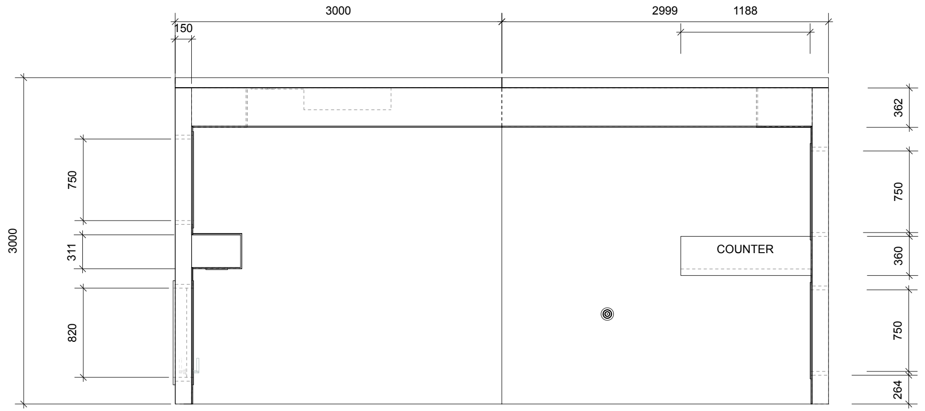
1 FLOOR PLAN OF SET BUILD Scale: 1:25
