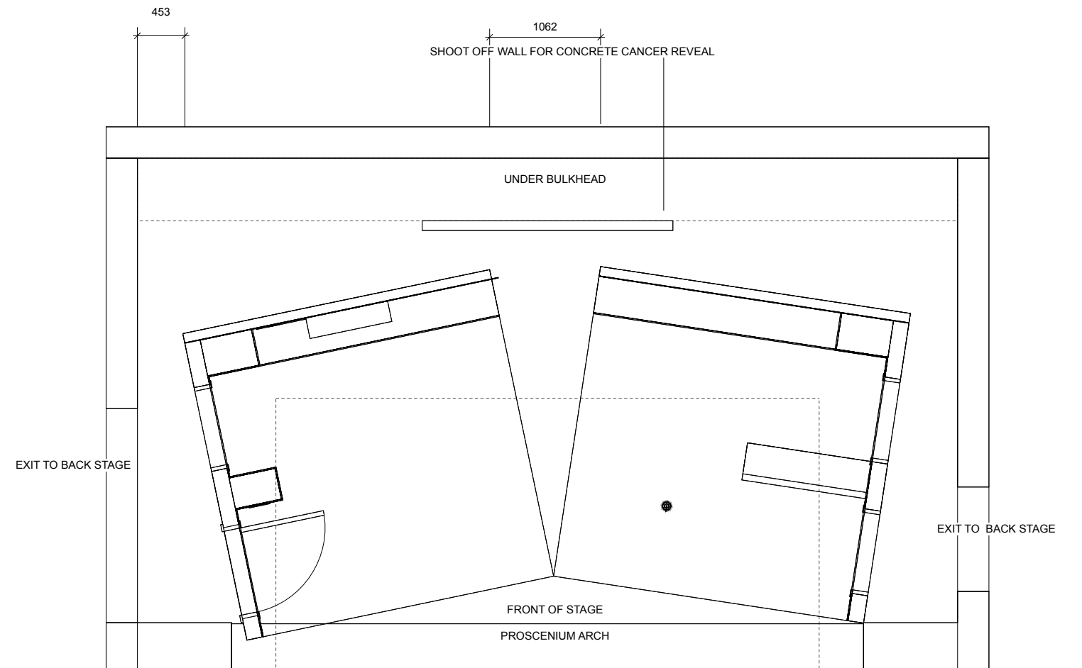
6 SITE PLAN - SET OPENED Scale: 1:25
