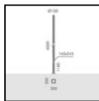
S.1486 H 4,0m Ø150mm CYLINDRICAL POLE WITH BASE
