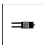
S.2407 POWER SUPPLY NOT DIMMABLE 14,4W 230Vac/24Vdc IP67 In: 240V Alternate Current Out: 24V Direct Current. The Total power of all connected luminaires may not be higher than the power of the driver. IP67 CLASS II SELV Dimensions: 79 x 38 x 25 mm. WE SUGGEST TO USE ONE SURGE PROTECTION DEVICE (S.2499) FOR EACH REMOTE DRIVER AT A DISTANCE OF NO MORE THAN 10m AWAY.
