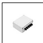
S.2404 POWER SUPPLY NOT DIMMABLE IN BOX 90W 230Vac/24Vdc IP55 MAX 5 OUTPUTS Dimensions: 260 x 240 x 100 mm. Cable IN: 2 with cable glands PG11 Cable OUT: 5 with cable glands PG11 IP55 CLASS II SELV The Total power of all connected luminaires may not be higher than the power of the driver. WE SUGGEST TO USE ONE SURGE PROTECTION DEVICE (S.2499) FOR EACH REMOTE DRIVER AT A DISTANCE OF NO MORE THAN 10m AWAY.
