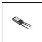
S.2411 POWER SUPPLY 0/1-10V 230V/700mA 17W o 230V/24V 15W IP68 230V/700mA Maximum power consumption: 17W or 230V/24V Frequency PWM : 240Hz Maximum power consumption: 15W Dimensions 121mmx53mmx26mm IP68 SELV CLASS II Warning!!! Always check the minimum Forward voltage (Vf min) of the fixtures that will be connected to this driver. WE SUGGEST TO USE ONE SURGE PROTECTION DEVICE (S.2499) FOR EACH REMOTE DRIVER AT A DISTANCE OF NO MORE THAN 10m AWAY.
