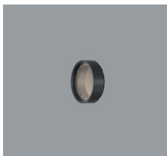
AC006008 Bread and Pastry Filter Filter holder: polymer, black, rotatable through 360°. Replacement without tools. Weight 0.03kg
