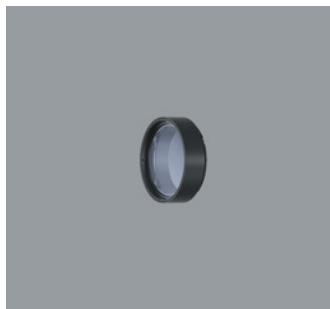
AC006013 Fish Filter Filter holder: polymer, black, rotatable through 360°. Replacement without tools. Weight 0.03kg
