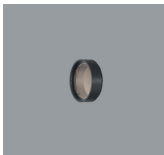
AC006010 Marbled Meat Filter Filter holder: polymer, black, rotatable through 360°. Replacement without tools. Weight 0.03kg
