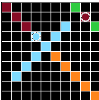
predicted
