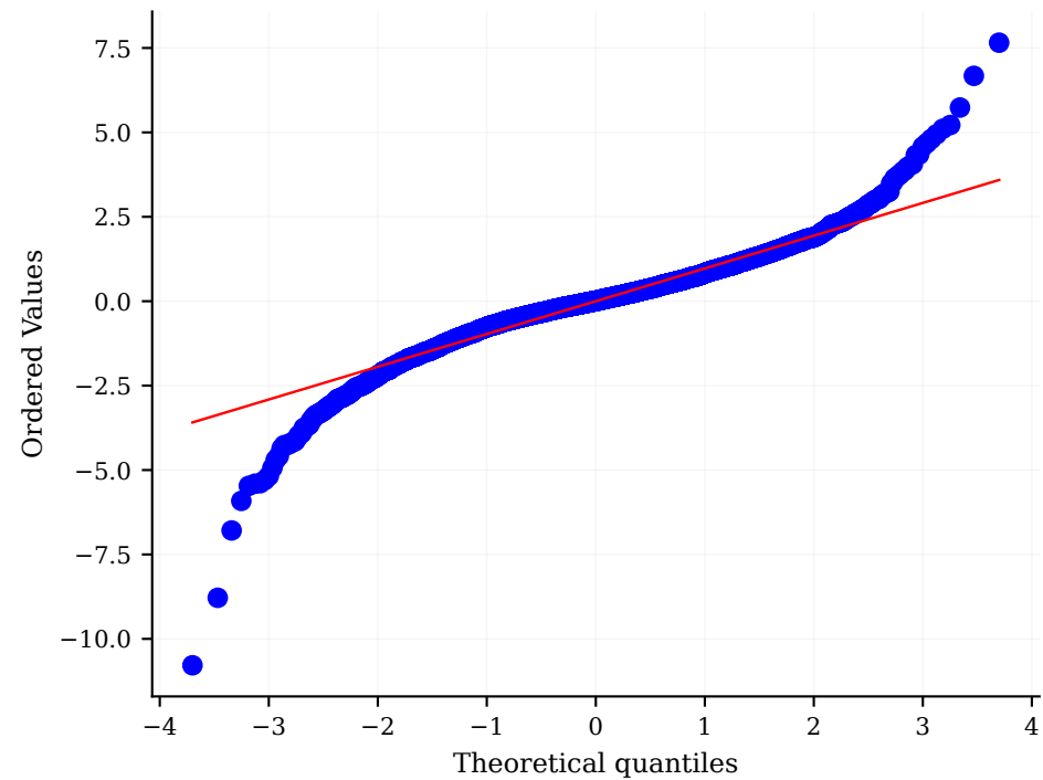
10Y Treasury (excess kurtosis = 2.47)
