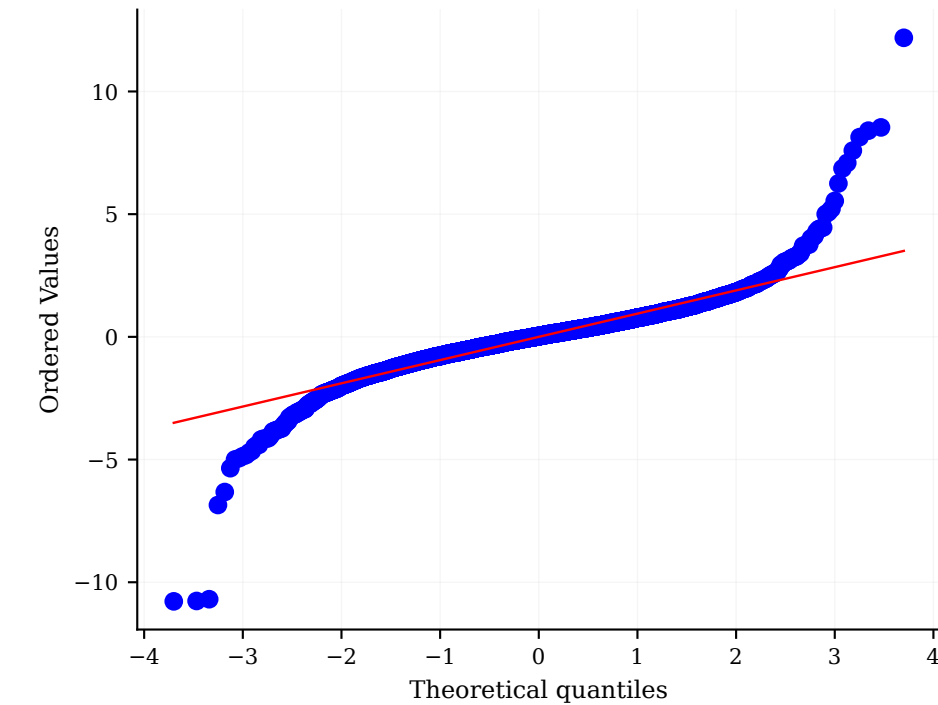
Oil (excess kurtosis = 15.76)
