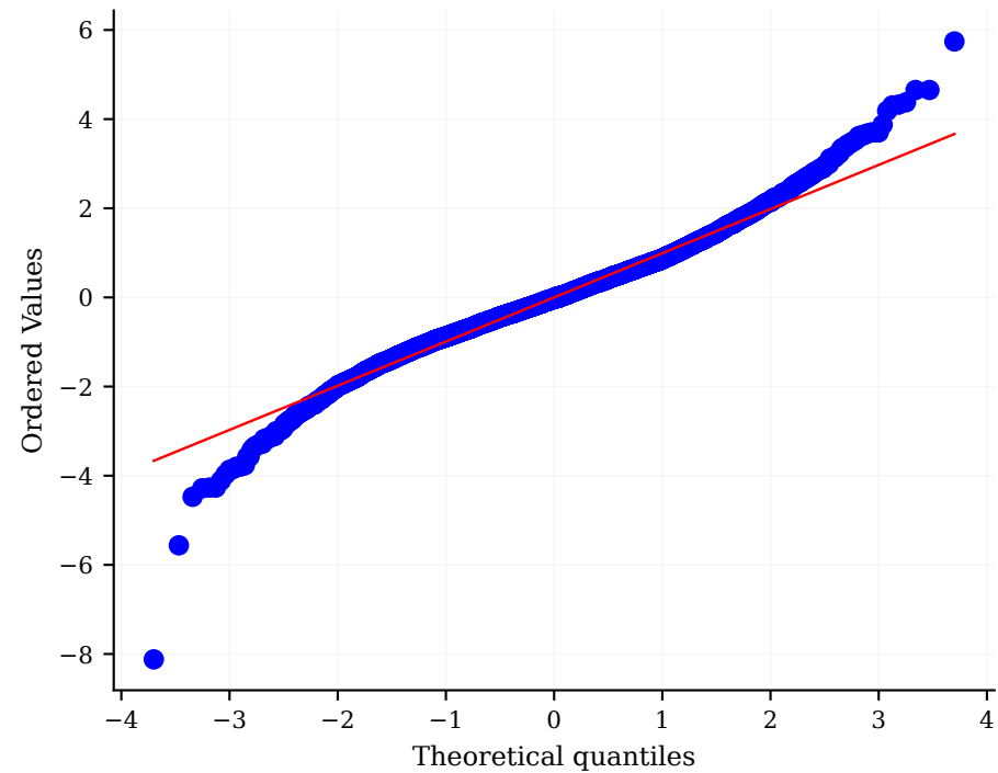
10Y Yield (excess kurtosis = 2.30)
