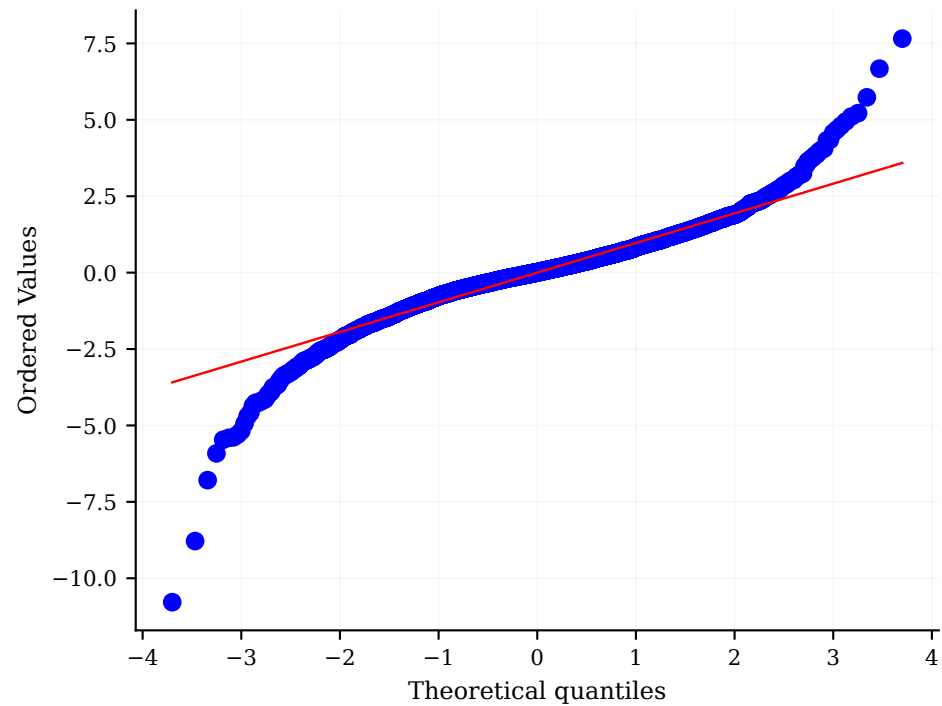
10Y Yield (excess kurtosis = 2.30)
