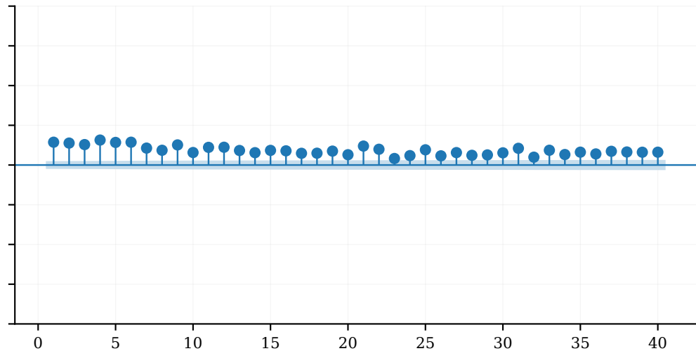
10Y Yield: ACF(r_t^2)
