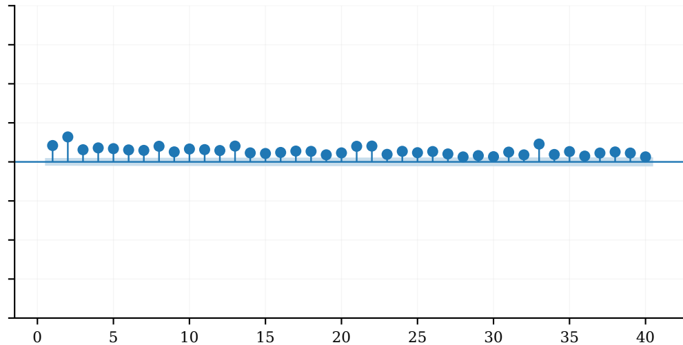
10Y Treasury: ACF(r_t^2)
