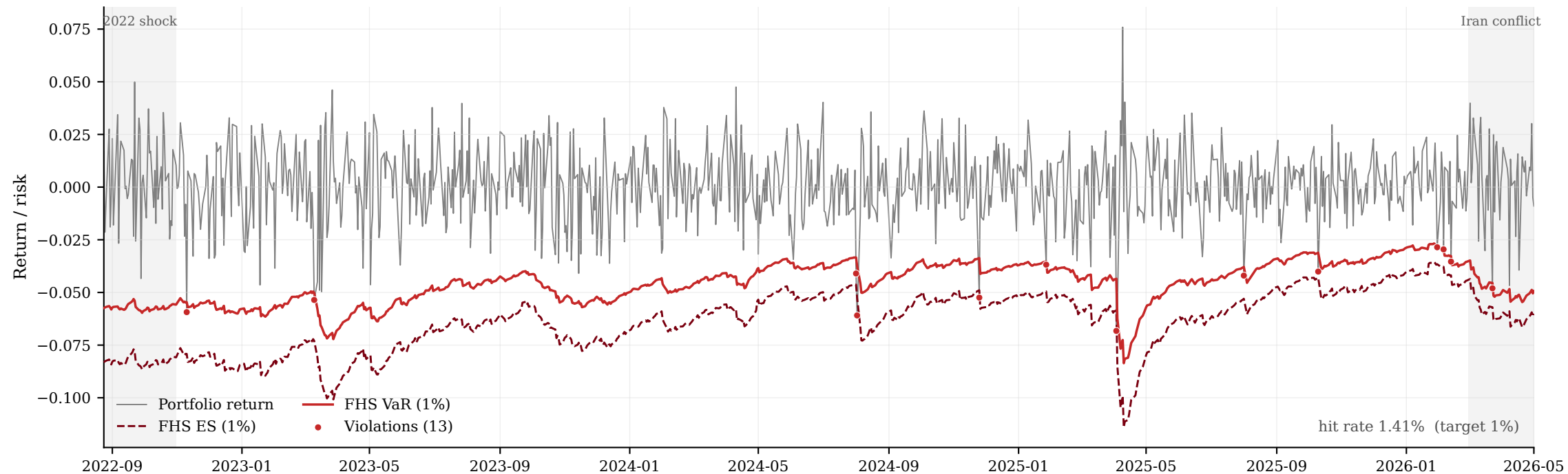
Asymmetric BEKK: one-step-ahead FHS VaR/ES (equal-weight portfolio)
