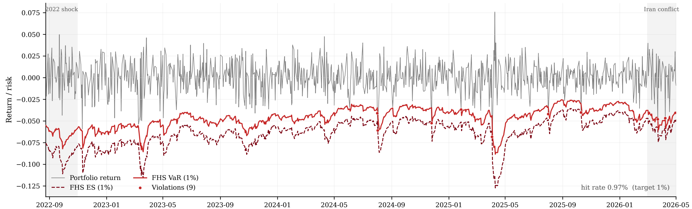
BEKK-LSTM (mix): one-step-ahead FHS VaR/ES
