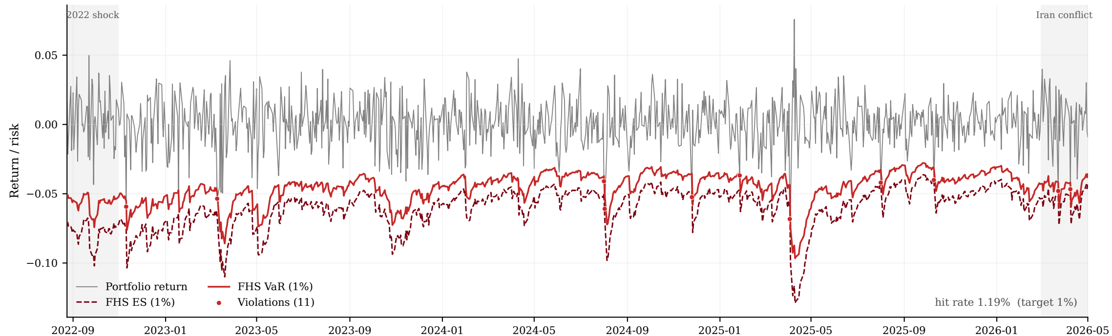
BEKK-LSTM (scalar): one-step-ahead FHS VaR/ES
