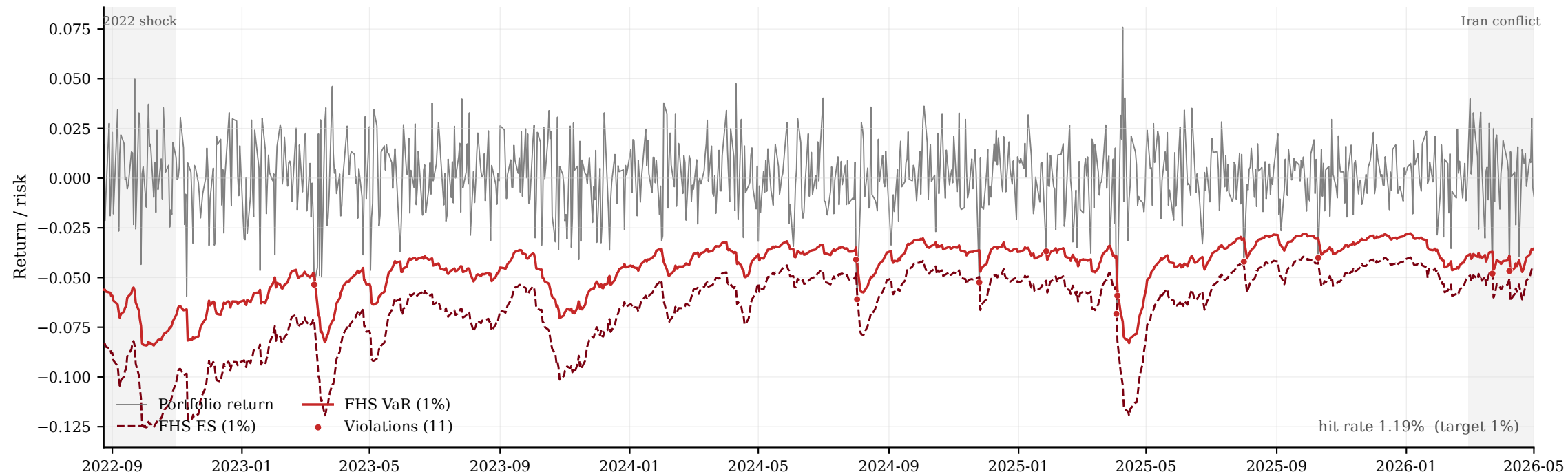
BEKK-LSTM (vector): one-step-ahead FHS VaR/ES
