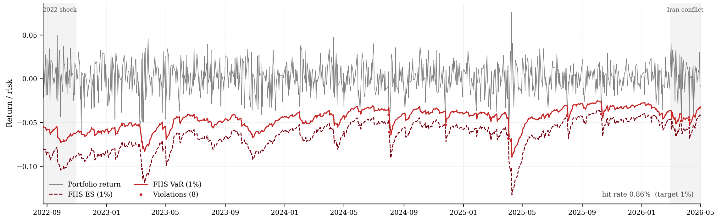
Neural-BEKK (asym. diag.): one-step-ahead FHS VaR/ES
