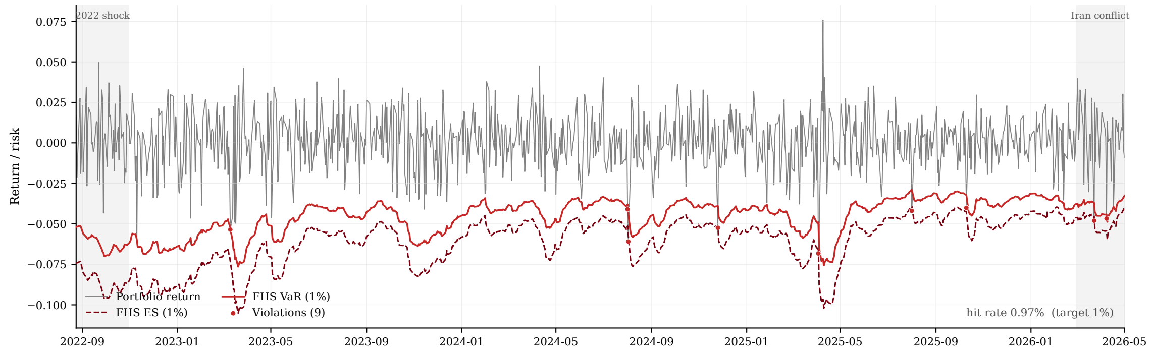
Neural-BEKK (asym. full): one-step-ahead FHS VaR/ES
