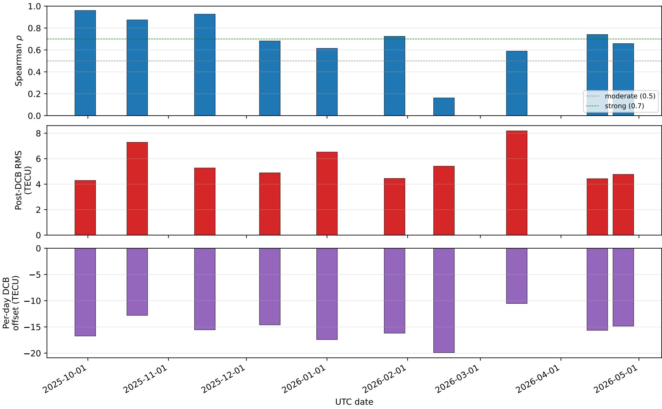
Vertical-TEC cross-validation against IGS GIM (N=10 days spanning the cruise)
