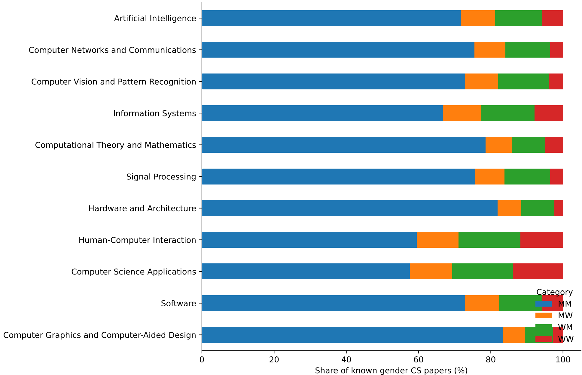
Gender composition across major Computer Science subfields
