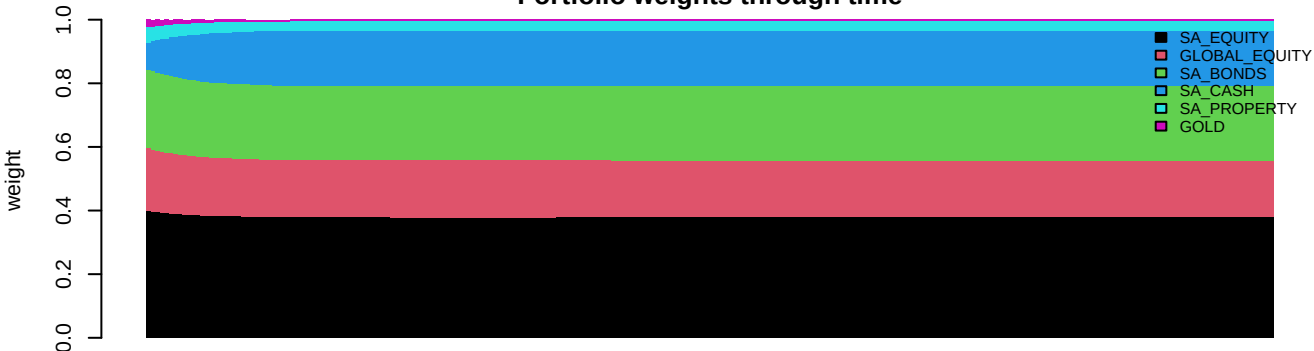
Portfolio weights through time
