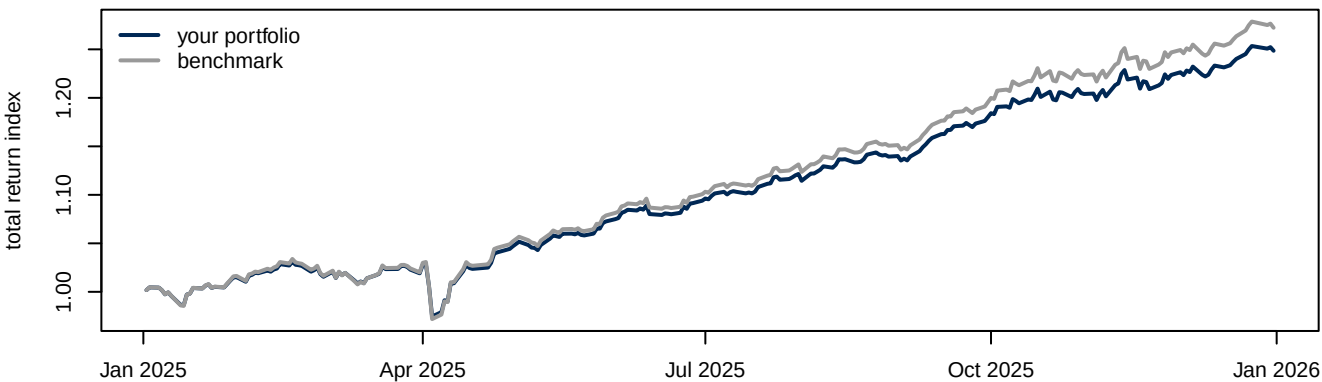
Total return: portfolio vs benchmark
