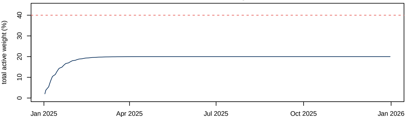
Total active weight
