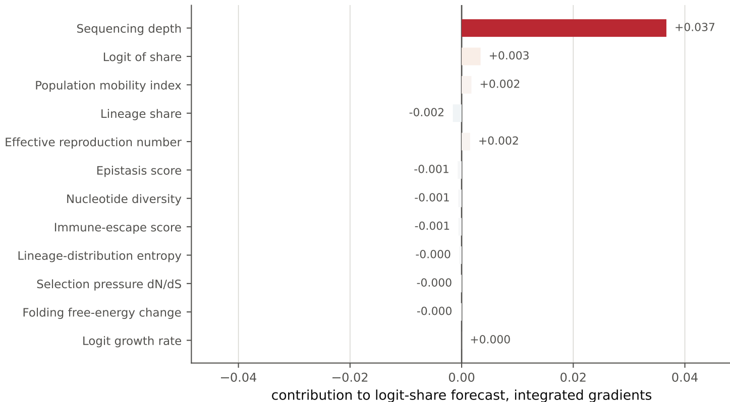
Figure 6 — feature attribution via integrated gradients
