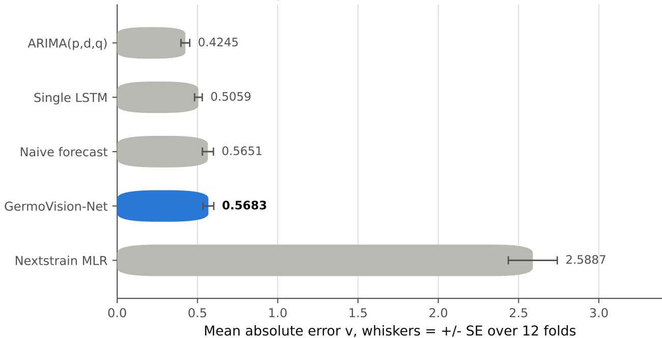
Figure 10 — MAE comparison against baseline models
