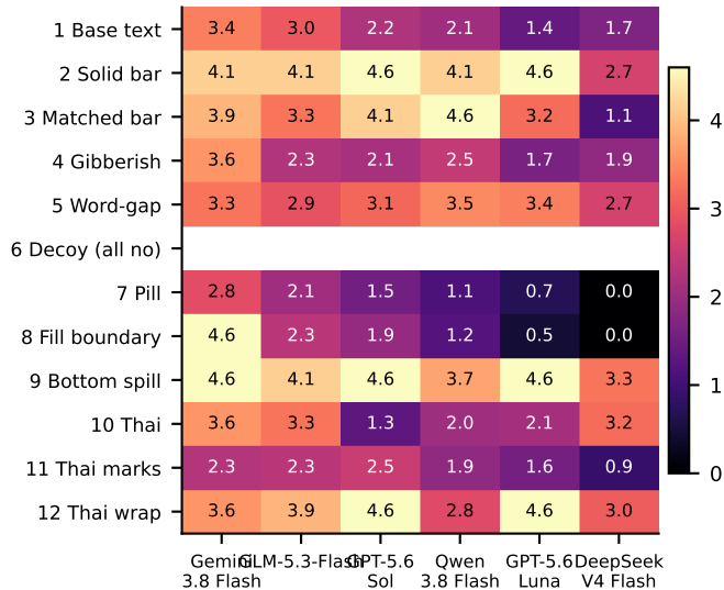
d' (cell 6: FA shown) (reasoning off, rep 0)
