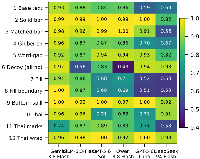
accuracy (reasoning off, rep 0)
