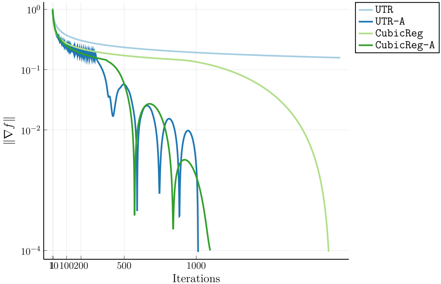
Nesterov's Lower Bound Function: n := 150, k := 50, p := 3
