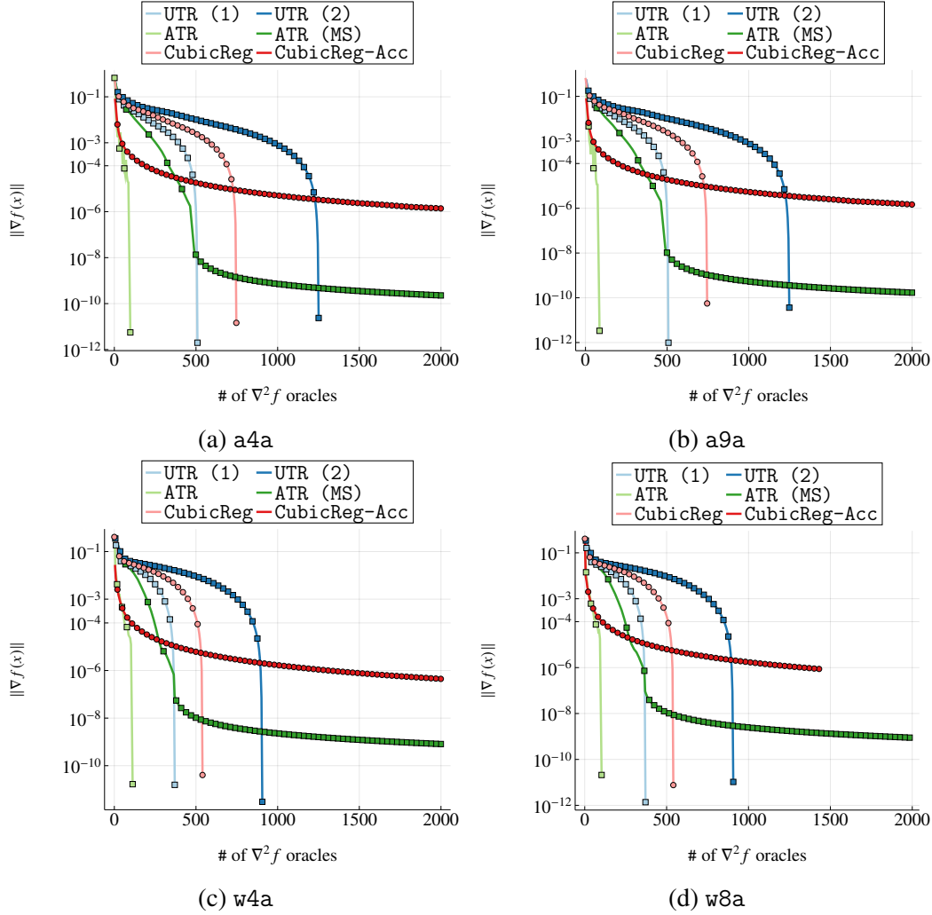
FIGURE 1. Logistic regression using the LIBSVM datasets fig.logistic regression
